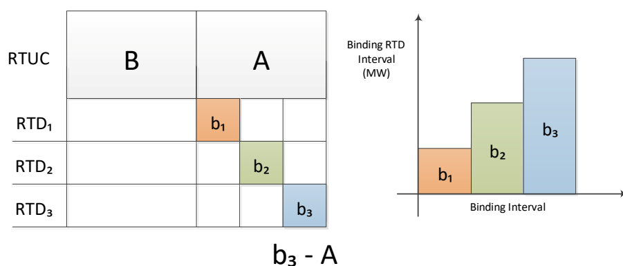
Figure 4: Histogram construction in FMM
